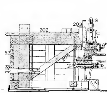
Fig. 415. Longitudinal Section.
